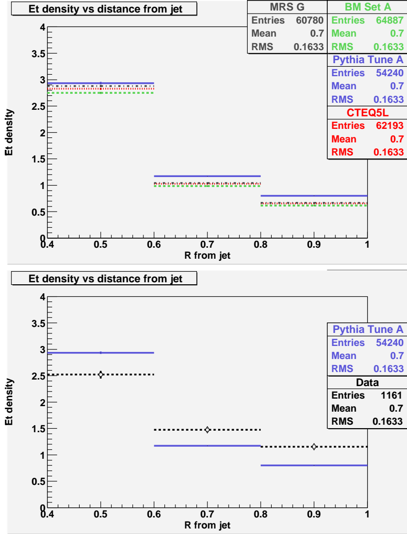
Figure 7: E_T density [GeV/(unit \eta - \phi )] as a function of distance from the jets in the Monte Carlo samples (top) and data (bottom). PYTHIA Tune A is also included on the data plot to facilitate comparison. On the Monte Carlo plot, the red (dotted) curve corresponds to CTEQ5L, the green (dashed) to BM Set A, the grey (dot-dash) to MRS G and the purple (solid) to PYTHIA Tune A.
