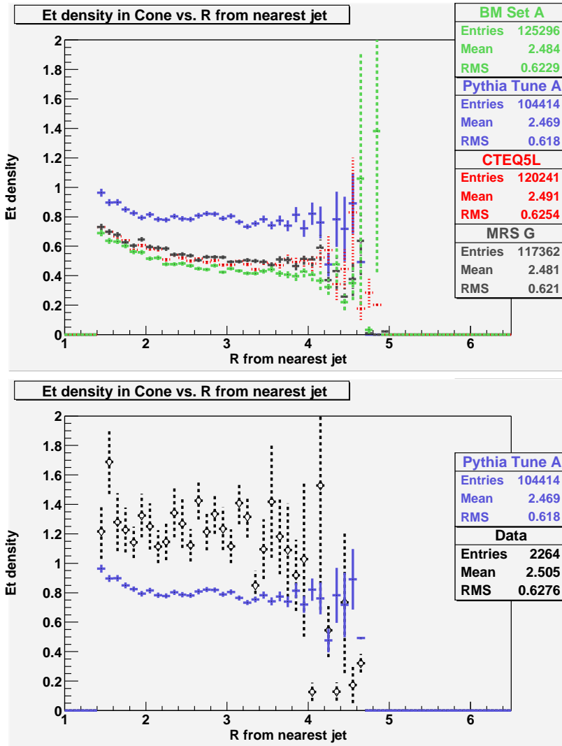
Figure 5: Dependence of the E_T density [GeV/(unit \eta - \phi )] in a cone of R = 0.4 on the displacement from the nearest jet in the Monte Carlo (top) and data (bottom). PYTHIA Tune A is also included on the data plot to facilitate comparison. On the Monte Carlo plot, the red (dotted) curve corresponds to CTEQ5L, the green (dashed) to BM Set A, the grey (dot-dash) to MRS G and the purple (solid) to PYTHIA Tune A.
