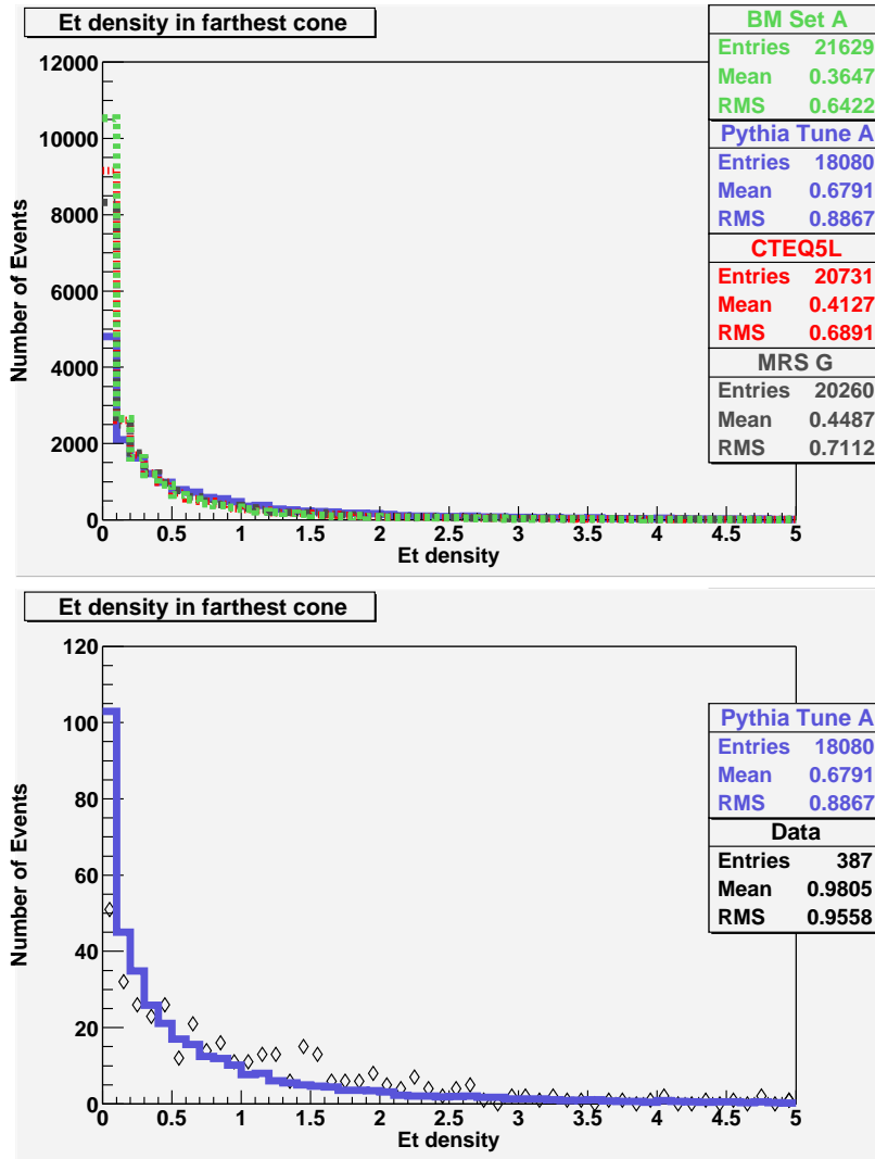
Figure 1: E_T density [GeV/(unit \eta - \phi )] in the cone farthest from all jets in an event. Monte Carlo samples are compared on the top and data is compared with PYTHIA Tune A on the bottom. The PYTHIA Tune A entries on the latter curve are scaled by a factor of 0.0214 to facilitate comparison with the data. On the Monte Carlo plot, the red (dotted) curve corresponds to CTEQ5L, the green (dashed) to BM Set A, the grey (dot-dash) to MRS G and the purple (solid) to PYTHIA Tune A.
