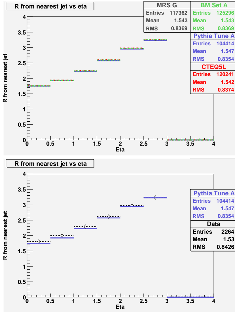
Figure 4: Average \eta dependence of the distance from the cone to the nearest jet in the Monte Carlo (top) and data (bottom). On the Monte Carlo plot, the red (dotted) curve corresponds to CTEQ5L, the green (dashed) to BM Set A, the grey (dot-dash) to MRS G and the purple (solid) to PYTHIA Tune A.
