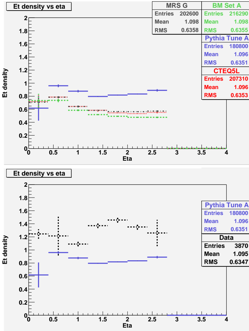
Figure 3: E_T density [GeV/(unit \eta - \phi )] vs \eta . Measurements are made in slices with width of two \eta towers and the density is measured outside R = 1.0 from all jets. Monte Carlo samples are shown on the top and data on the bottom. PYTHIA Tune A is also included on the data plot to facilitate comparison. On the Monte Carlo plot, the red (dotted) curve corresponds to CTEQ5L, the green (dashed) to BM Set A, the grey (dot-dash) to MRS G and the purple (solid) to PYTHIA Tune A.
