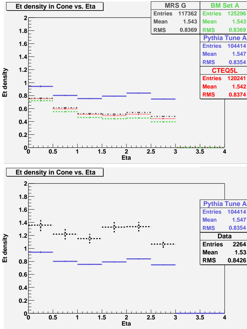
Figure 2: E_T density [GeV/(unit \eta - \phi )] in cones of R = 0.4 vs \eta . Monte Carlo samples are shown on the top and data on the bottom. PYTHIA Tune A is also included on the data plot to facilitate comparison. On the Monte Carlo plot, the red (dotted) curve corresponds to CTEQ5L, the green (dashed) to BM Set A, the grey (dot-dash) to MRS G and the purple (solid) to PYTHIA Tune A.
