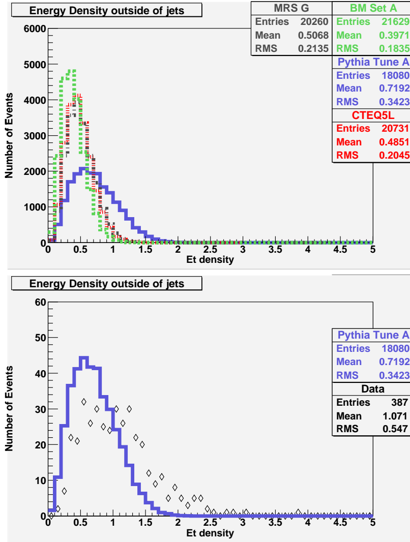
Figure 6: E_T density [GeV/(unit \eta - \phi )] in entire \eta - \phi space excluding the region that is within R=1.0 from any jet's centroid in the Monte Carlo samples (top) and data (bottom). PYTHIA Tune A is also included on the data plot to facilitate comparison. The PYTHIA Tune A entries on the latter curve are scaled by a factor of 0.0214 to facilitate comparison with the data. On the Monte Carlo plot, the red (dotted) curve corresponds to CTEQ5L, the green (dashed) to BM Set A, the grey (dot-dash) to MRS G and the purple (solid) to PYTHIA Tune A.
