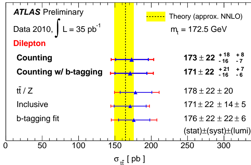
Figure 9.1: The \sigma_{t\bar{t}} cross section measurements presented in the thesis compared to other approaches. The measurement labeled as “ b -tagging fit” is the result from this thesis. The yellow bar reflects the uncertainty on the theoretical prediction, which includes some of the NNLO corrections supplemented by soft gluon resummation at the next-to-next-to-leading-logarithm accuracy.
