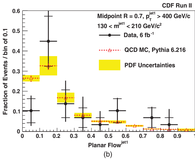
FIG. 15 (color). The normalized planar flow distribution for jets with p_T > 400 GeV/ c and |\eta| \in (0.1, 0.7) reconstructed with the R = 0.7 MIDPOINT cone algorithm. We have not rejected t\bar{t} events and have not placed any constraint on the jet mass in (a). The distribution after top-quark rejection and requiring m^{\text{jet}1} \in (130, 210) GeV/ c^2 is shown in (b). Data points are shown with statistical and systematic uncertainties. Results from the PYTHIA QCD prediction (red triangles) with the PDF uncertainties (yellow bars) are overlaid.
