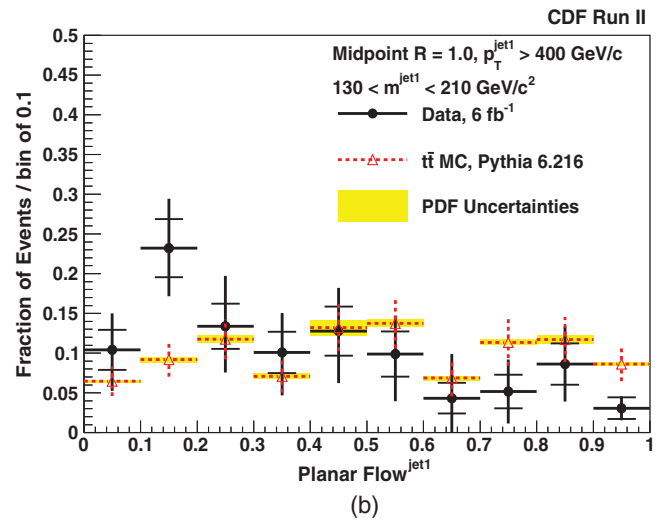
FIG. 16 (color). The normalized planar flow distribution for jets with p_T > 400 GeV/ c and |\eta| \in (0.1, 0.7) reconstructed with the R = 1.0 MIDPOINT cone algorithm. We have rejected t\bar{t} events and have required that m^{\text{jet}1} \in (130, 210) GeV/ c^2 . Data points are shown with statistical and systematic uncertainties. Overlaid in (a) are results from the PYTHIA QCD prediction (red triangles) with the PDF uncertainties (yellow bars). Overlaid in (b) are results from the PYTHIA MC prediction for the leading jet in t\bar{t} MC events (red triangles) with the PDF uncertainties (yellow bars).
