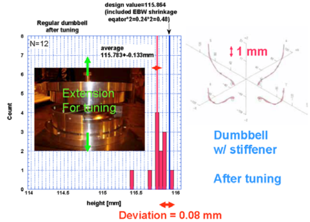
Figure 3: Dimensional measurements of dumbbells with stiffener-ring after tuning. Left-hand side: height measurement and height tuning by a special jig. Right-hand side: 3D measurement of dumbbell-cup. Black-curve is design shape and the red-lines denote the deviations from the design curve.
