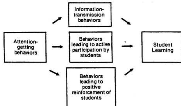
FIGURE 1 Relationships among four categories of classroom teaching behavior
